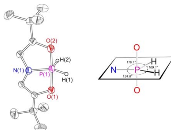
Figure 3. (Left) Thermal ellipsoid plot (50%) of 3 . Hydrogen atoms on carbon omitted for clarity. Selected bond distances (Å) and angles (deg): P(1)–N(1) = 1.676(2); P(1)–O(1) = 1.721(1); P(1)–O(2) = 1.699(1); P(1)–H(1) = 1.29(2); P(1)–H(2) = 1.31(2); O(1)–P(1)–O(2) = 170.5(1) ; N(1)–P(1)–H(1) = 134.8(1) ; N(1)–P(1)–H(2) = 116.1(1) ; H(1)–P(1)–H(2) = 109.1(2) . (Right) Schematic illustrating bond angles.
